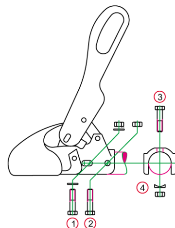
croquis 3: raccordement
